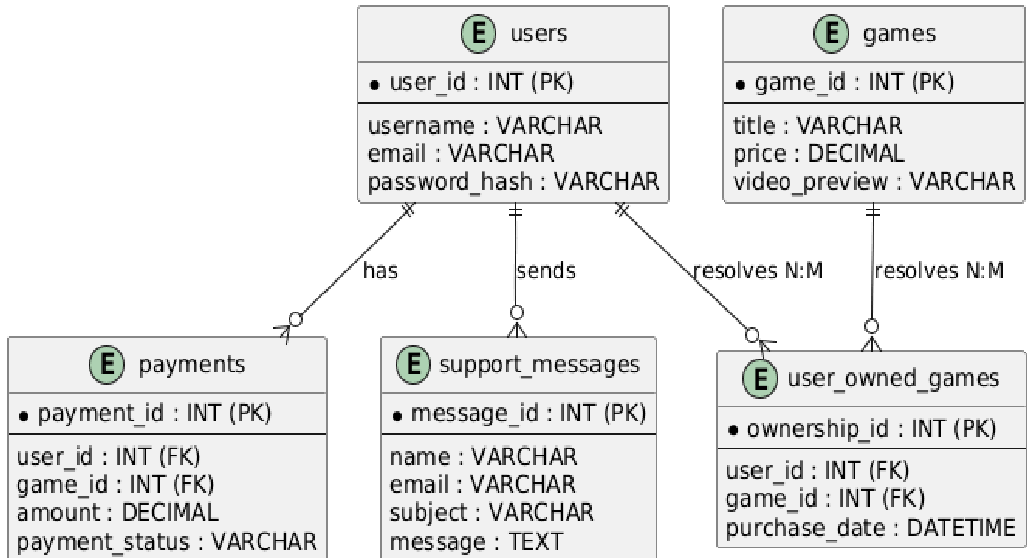
NexGenPlayz E-R Diagram
