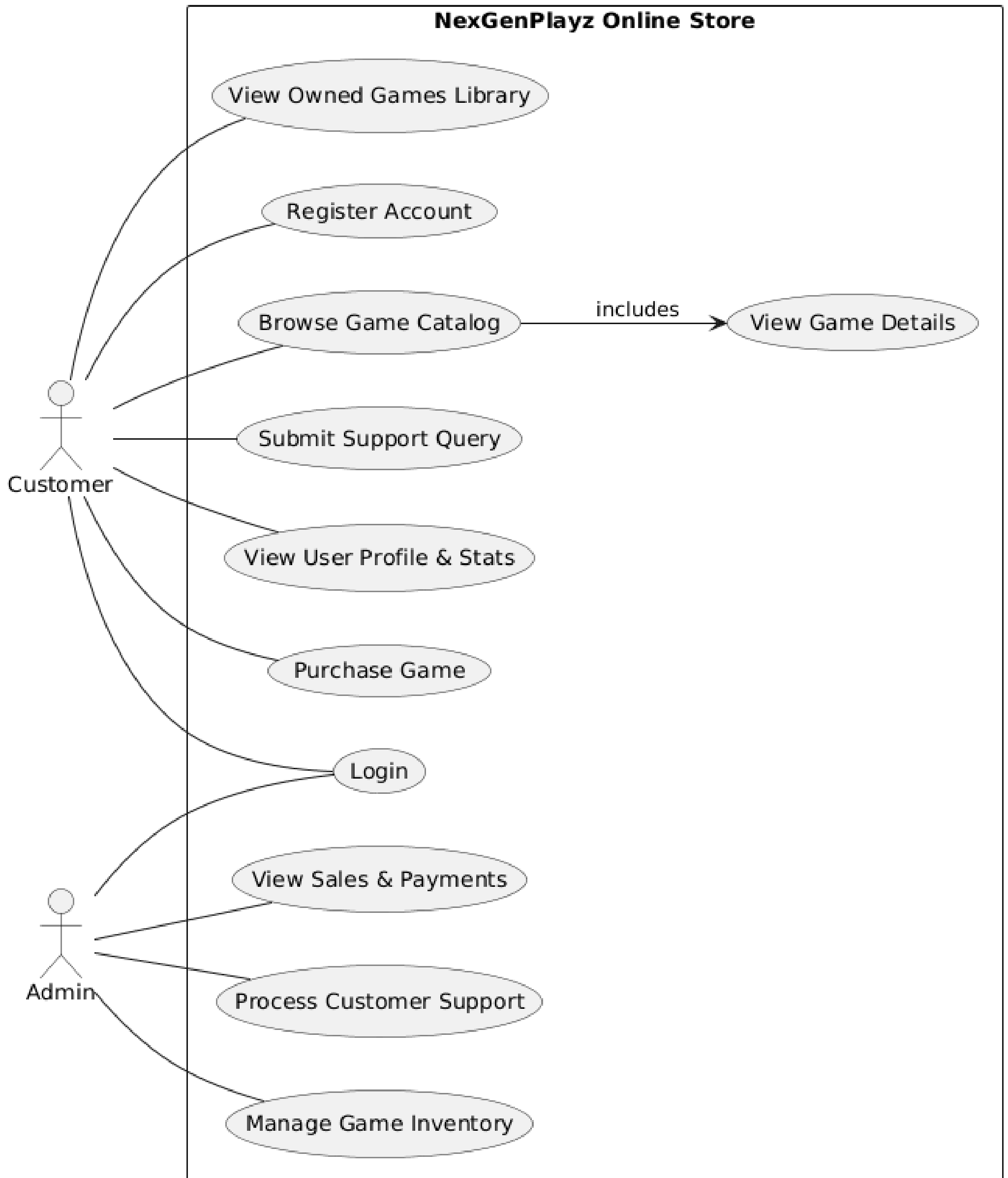
NexGenPlayz Use Case Diagram
